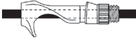
GRAPHITE BLANK EXPOSED CASTING REEL SEATS
